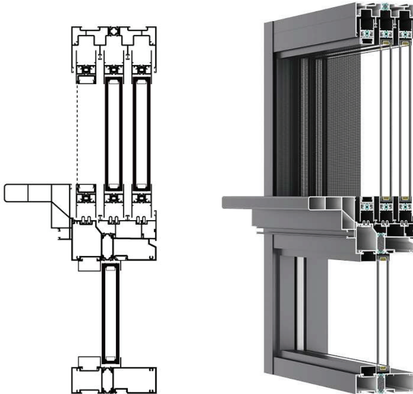
Concealed Sash
